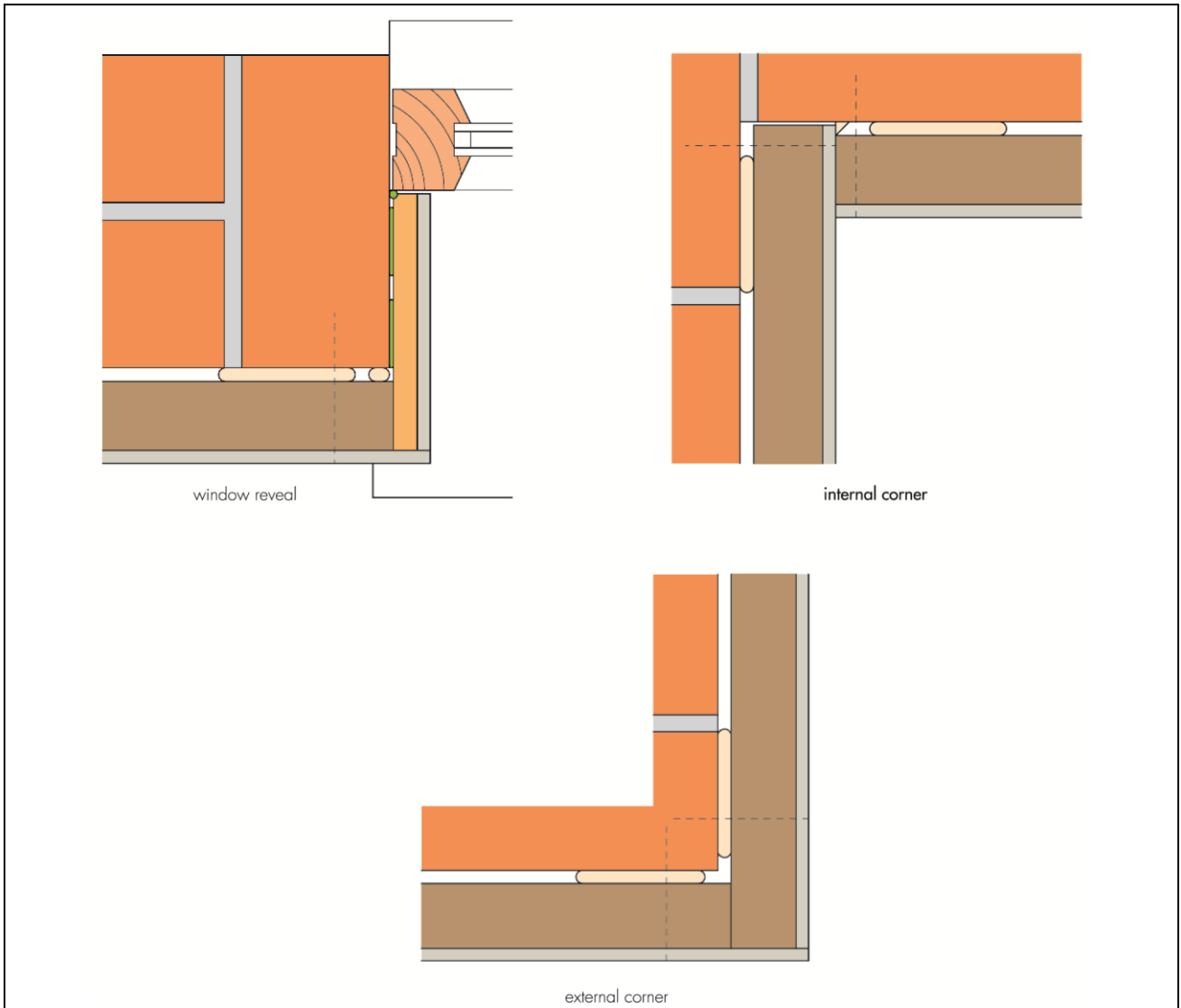
Figure 2 DriLyner TL construction details
